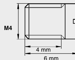
Throttle screw for FF 4-12/30/60/120/250
